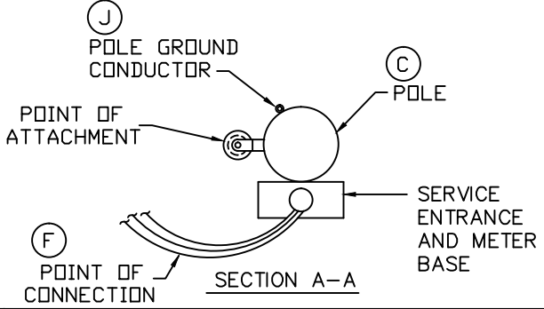
PERMANENT METER POLE
